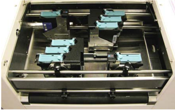
EIGHT PRINTHEADS
